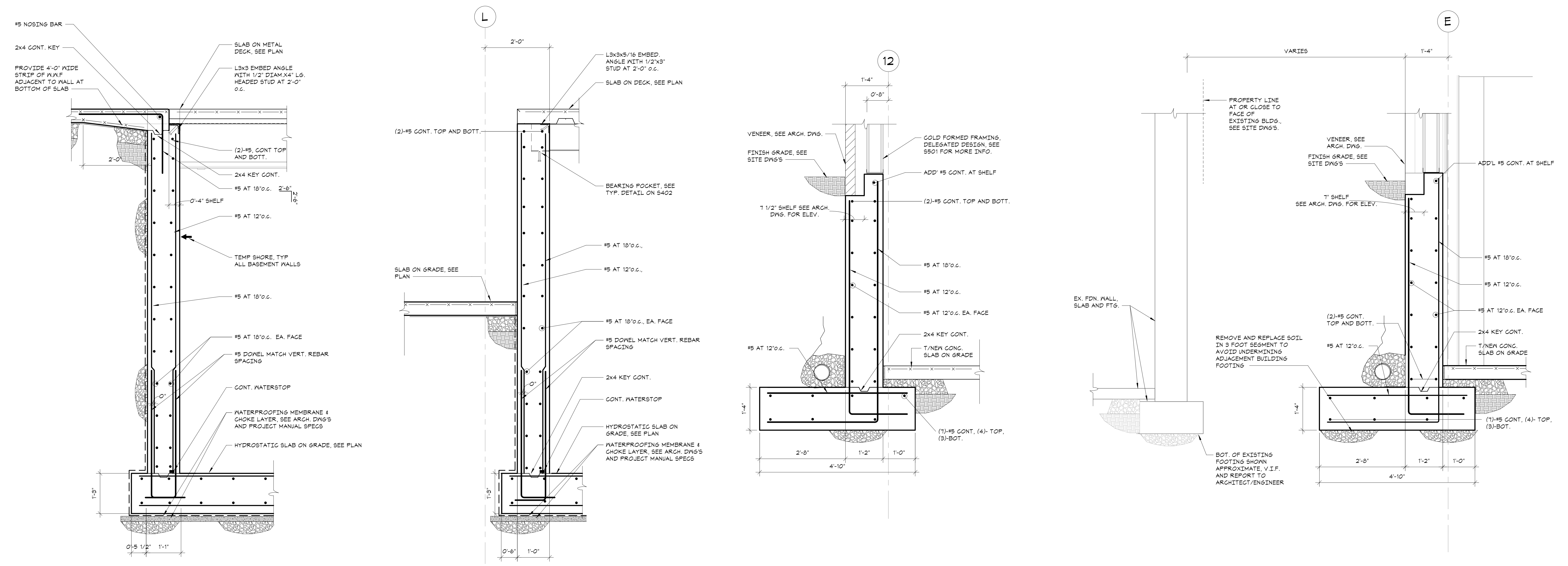
6 SECTION 3/4" = 1'-0" 7 SECTION 3/4" = 1'-0" 8 SECTION 3/4" = 1'-0" 9 SECTION 3/4" = 1'-0"
