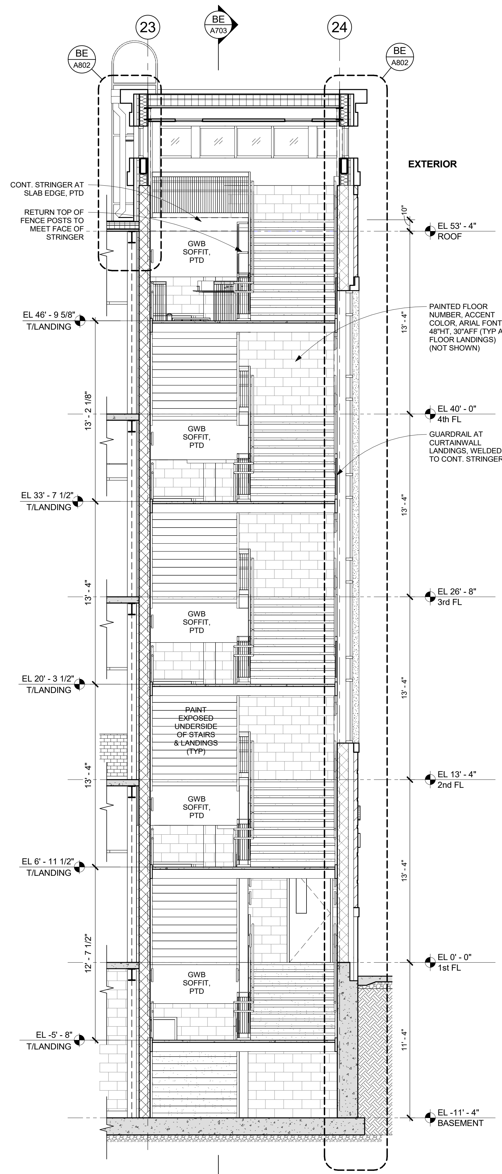
BN STAIR B - SECTION N 1/4" = 1'-0"
