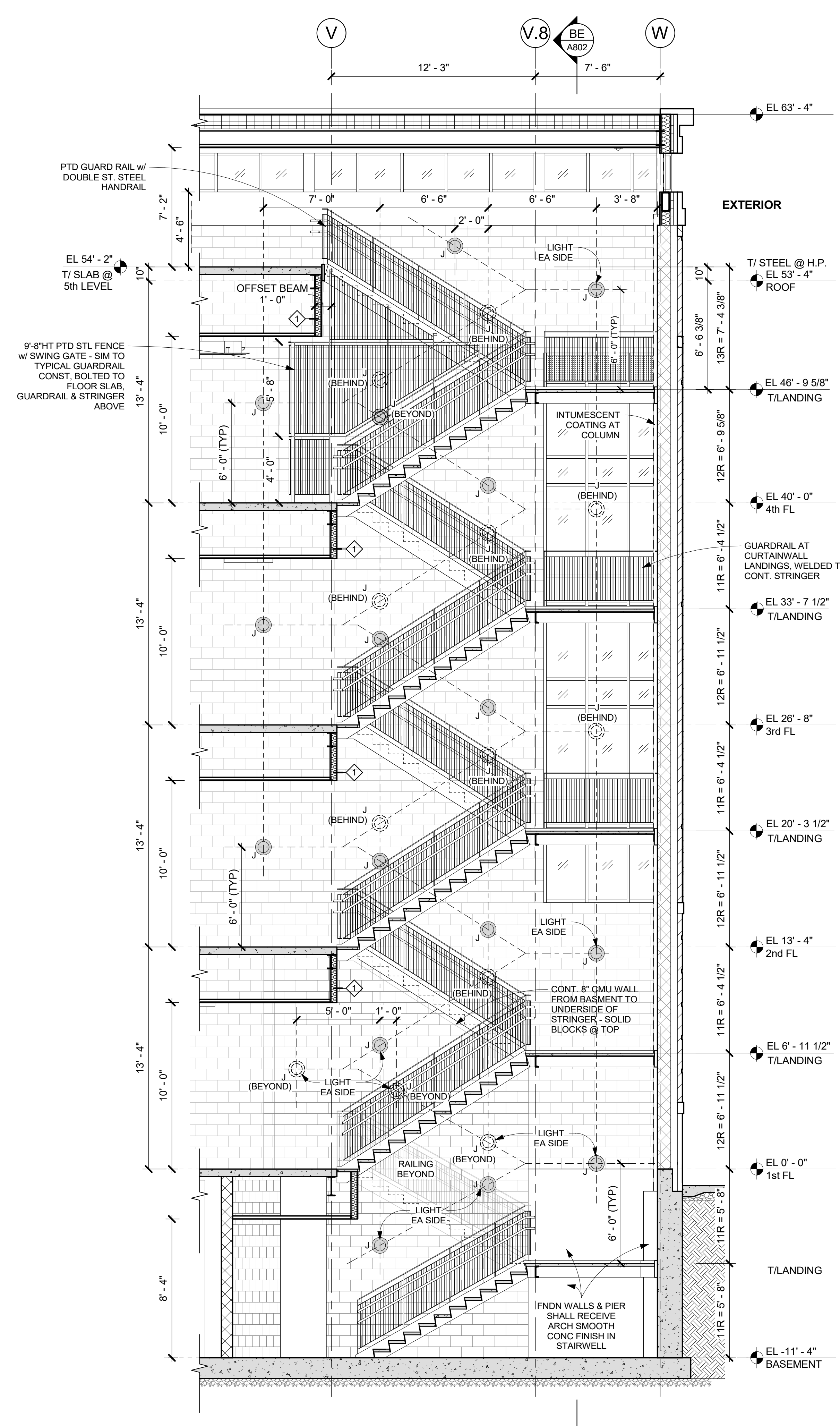
BE STAIR B - SECTION E 1/4" = 1'-0"
