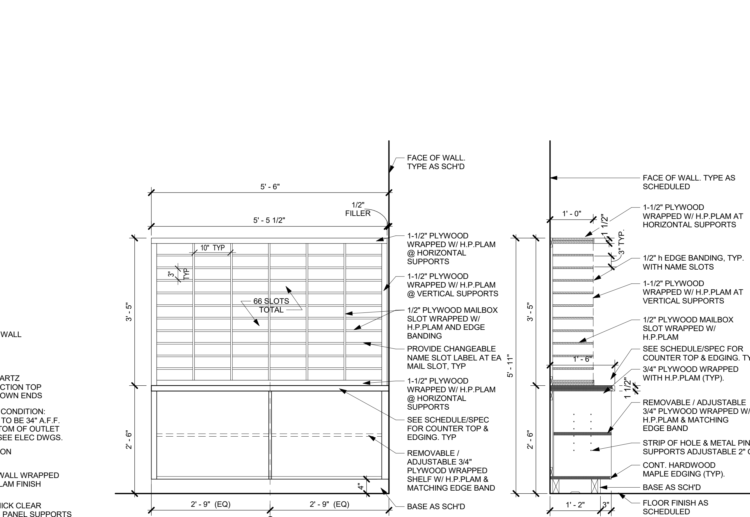
15 TYPICAL MAILBOX COUNTER 3/4" = 1'-0"
