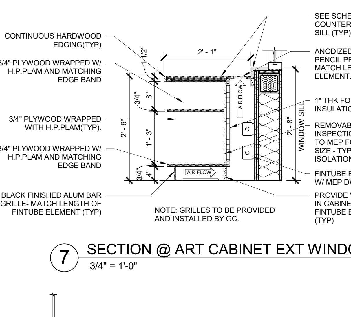
5 SECTION @ BASE CABINET 3/4" = 1'-0"
