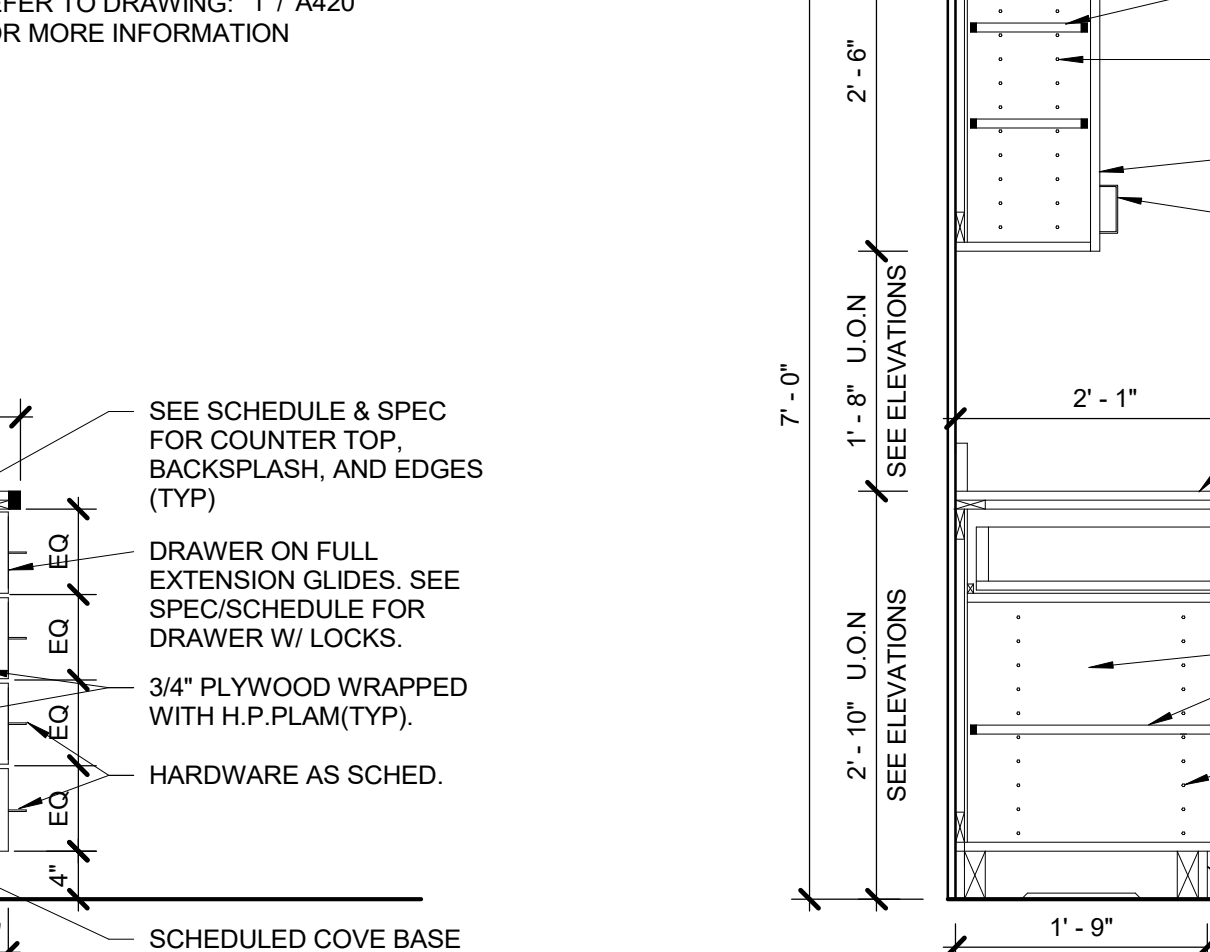
1 TYP. SECTION @ BASE & WALL CABINET 3/4" = 1'-0"
