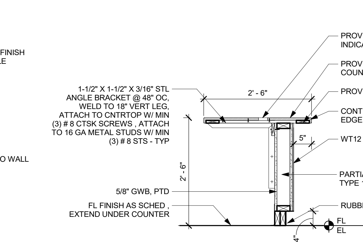
10 SECTION @ CIRCULATION DESK 2 3/4" = 1'-0"
