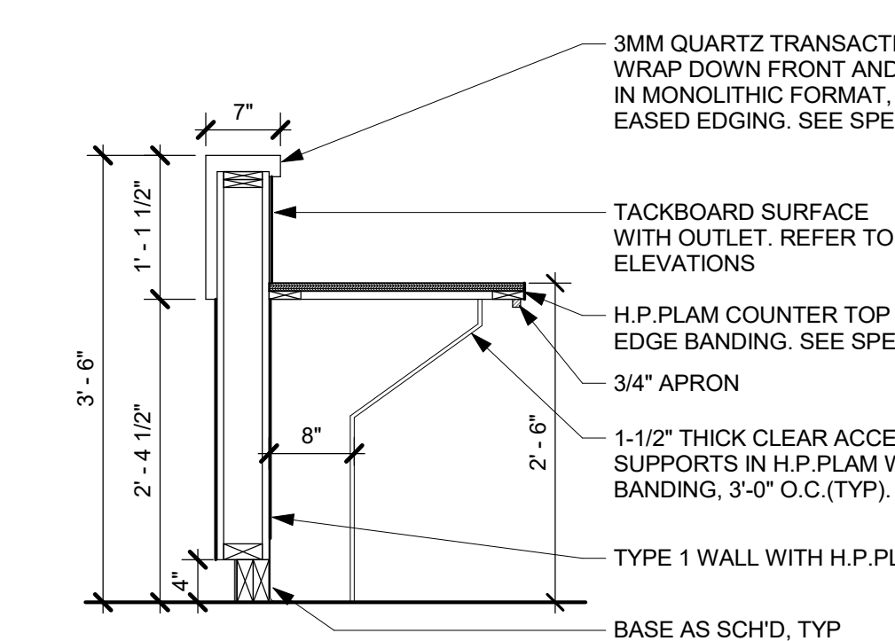
17 SECTION 1 @ MAIN OFFICE DESK 3/4" = 1'-0"
