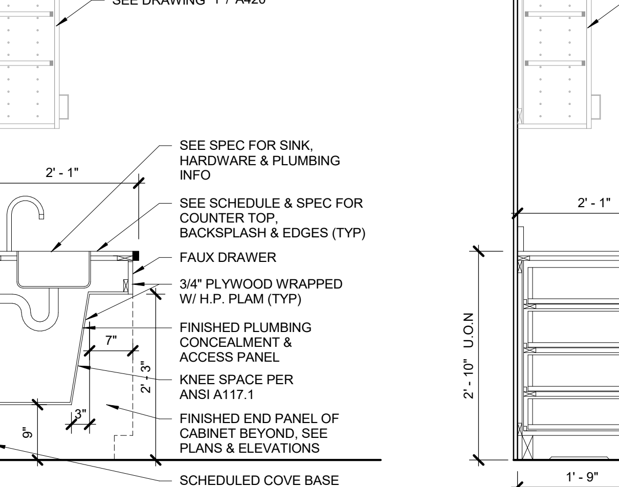
2 SECTION @ CABINET W/ DRAWERS 3/4" = 1'-0"
