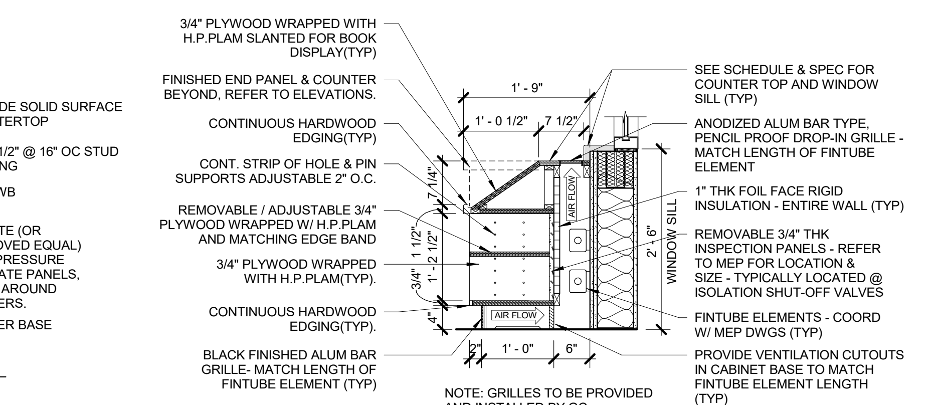
8 SECTION @ BOOK DISPLAY CABINET @ EXT WINDOW SILL 3/4" = 1'-0"
