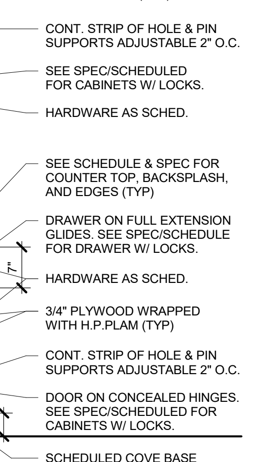
4 SECTION @ CHILD SINK W/ CABINET 3/4" = 1'-0"
