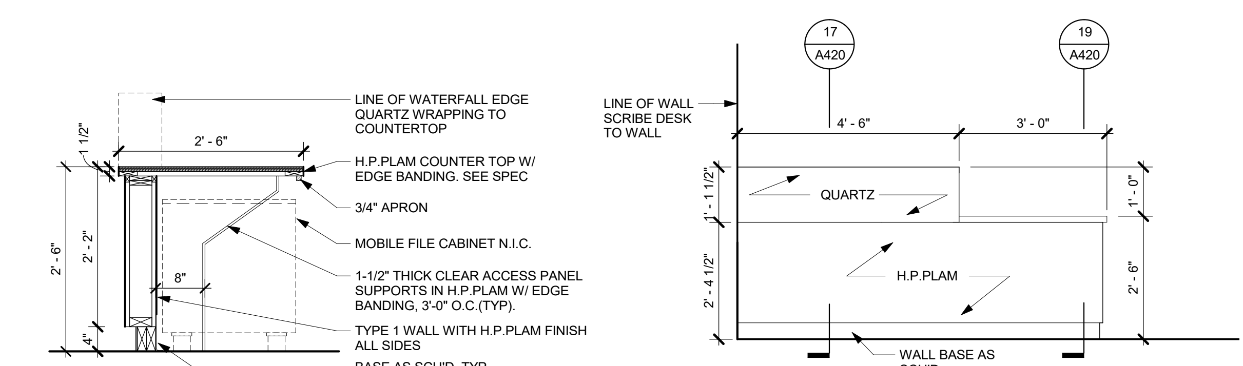
19 SECTION 2 @ MAIN OFFICE DESK 3/4" = 1'-0"
