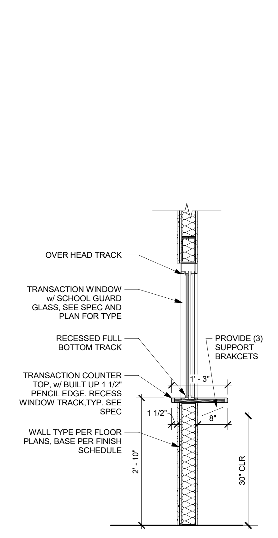
13 TYP TRANSACTION WINDOW 3/4" = 1'-0"
