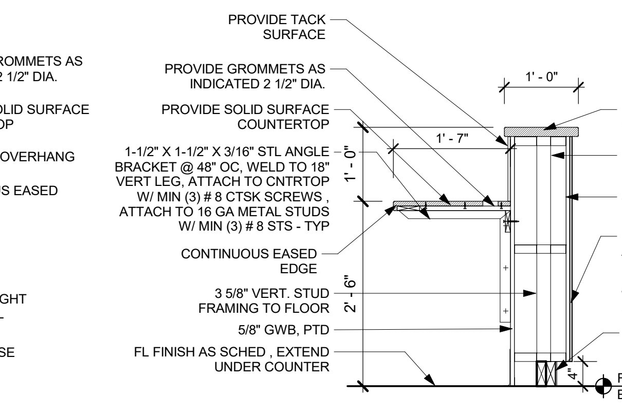
9 SECTION @ CIRCULATION DESK 3/4" = 1'-0"
