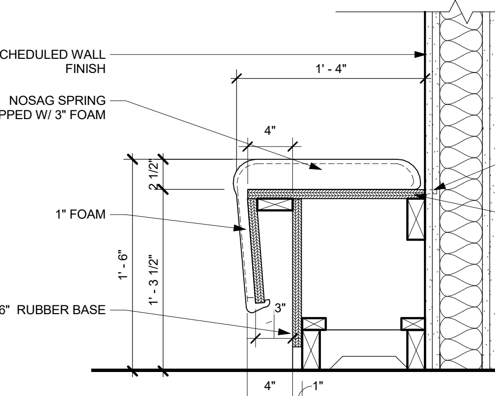
12 SECTION THRU UPHOLSTERED BENCH 1 1/2" = 1'-0"
