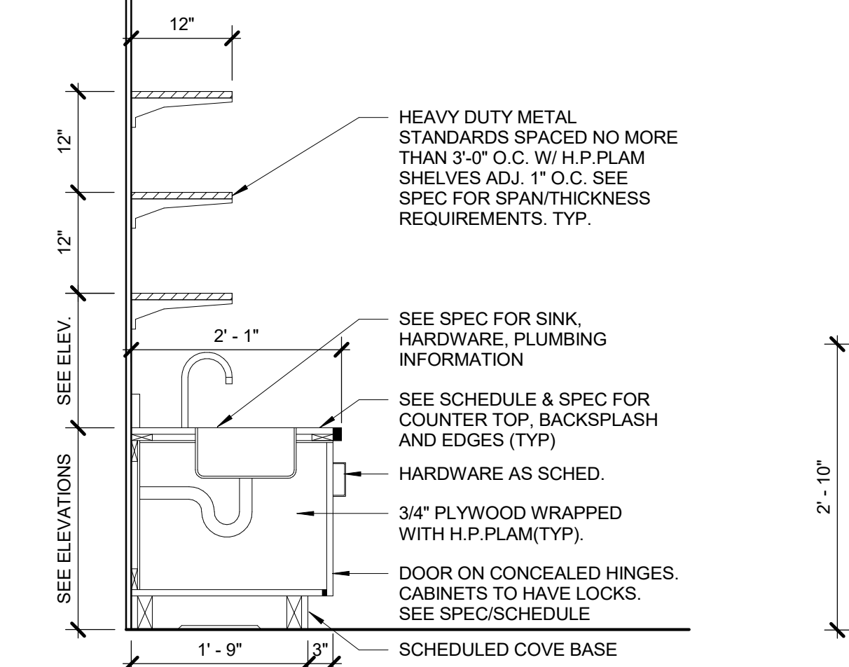
3 SECTION @ ADA SINK 3/4" = 1'-0"
