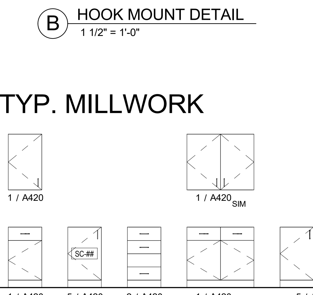
1 TYP. SECTION @ BASE & WALL CABINET 3/4" = 1'-0"
