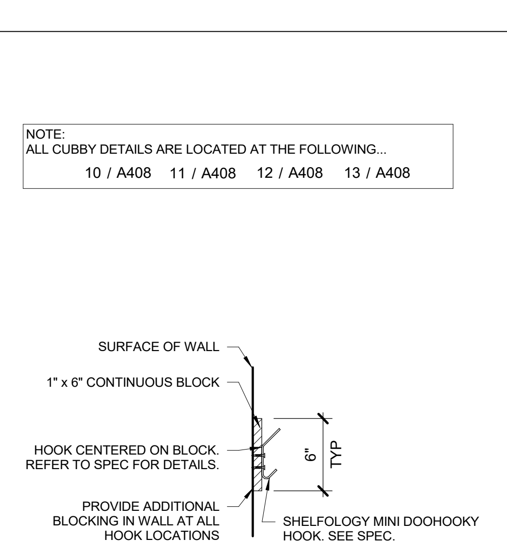
7 SECTION @ ART CABINET EXT WINDOW SILL 3/4" = 1'-0"
