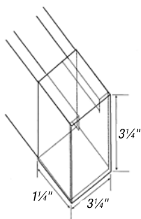
H804 NEOP WH 1 1/4" x 3/4" White Plastisol End-Cap
