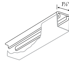
AB-844* Steel Closure Strip AB-844-PC* Plastic Closure Strip When used as a raceway channel, it is normally installed with the slot up and after wiring is complete, the closure strip is installed. For all channels. Standard lengths 10 ft.
