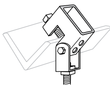
US562 Beam Clamp with Swing Hanger ½" screw included. Rod size: ½" Design load 800 lbs.
