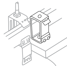
A854L Channel Hanger Long type for all series channel. Illustration showing A-854-L with nut and bolt furnished to attach to fluorescent fixture. Long type for all series channel.
