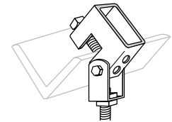
U563 Beam Clamp with Swing Hanger ⅝" set screw included. Rod sizes: ⅝" Design load 540 lbs.
