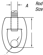
M-117 MI Socket for S Split Ring Hanger Sizes ¾" through ¾" Rod Federal Type 16 SP69 Type 16
