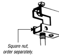
U563 Beam Clamp Optional Use ⅝" set screw included. Rod size: ⅝" Design load 400 lbs.
