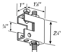
U563 Beam Clamp ⅝" set screw included. Rod size: ⅝" Design load 250 lbs.
