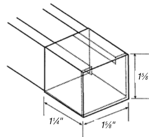
A804 NEOP WH 1 1/4" x 1 5/8" White Plastisol End-Cap
