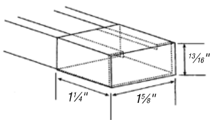
B 804 NEOP WH 1 1/4" x 1 3/16" White End-Cap
