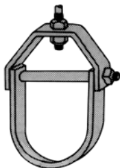
C-710 Series Standard Clevis
