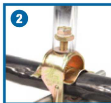
2 Using a power tool fitted with a ¾" (16mm) socket, tighten lock nut...
