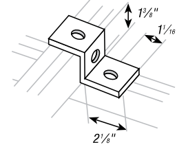
CAT. NO. C209 For attaching "C" series channel.
