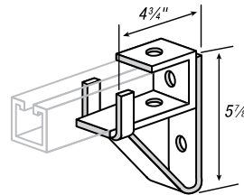
S247 Design Moment (channel upright as shown) When supported by A-1,200 5,250 inch lbs. A-1,400 3,650 inch lbs. Applies to fitting only, not to the arm. For A-1,200 B-1,202 A-1,400 B-1,402
