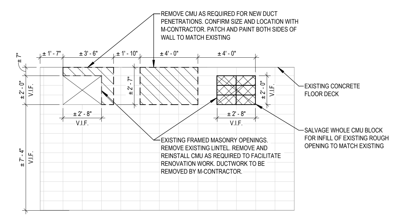
3 STORAGE 170A - ELEVATION SCALE: 1/4" = 1'-0"
