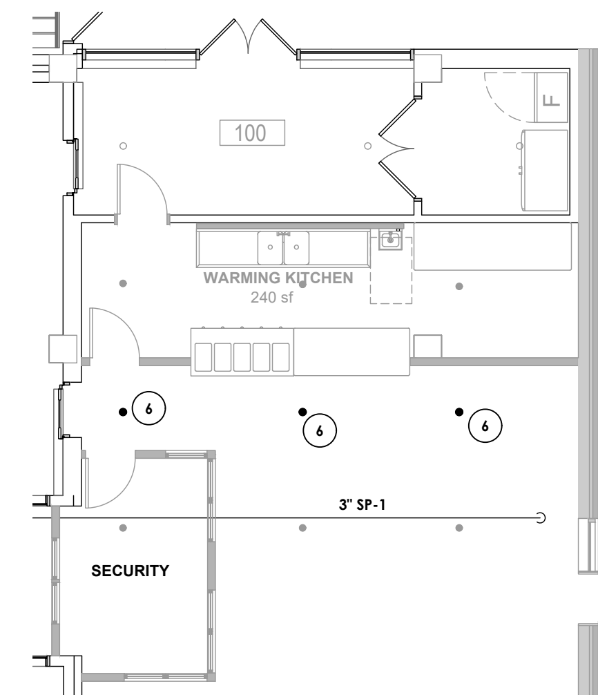
11 WARMING KITCHEN PLUMBING NEW WORK P201 SCALE: 1/8" = 1'-0"
