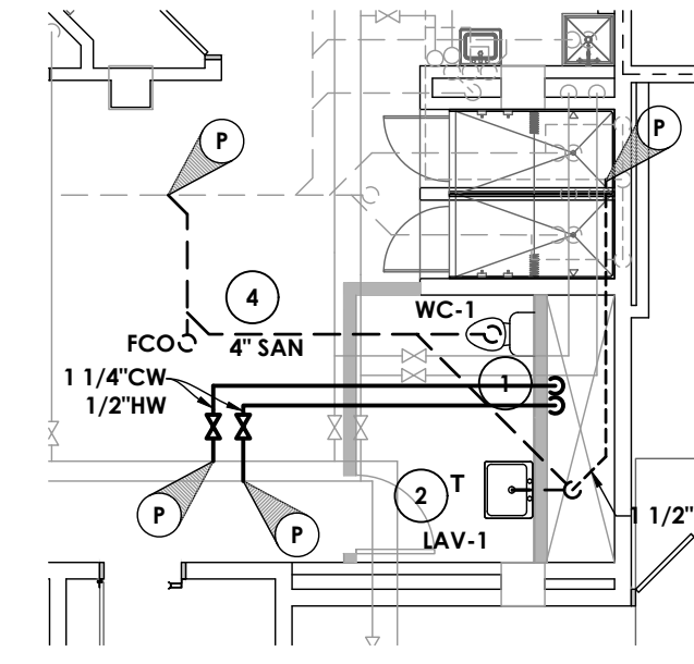
3 NEW TOILET ROOM PLUMBING NEW WORK P201 SCALE: 1/8" = 1'-0"
