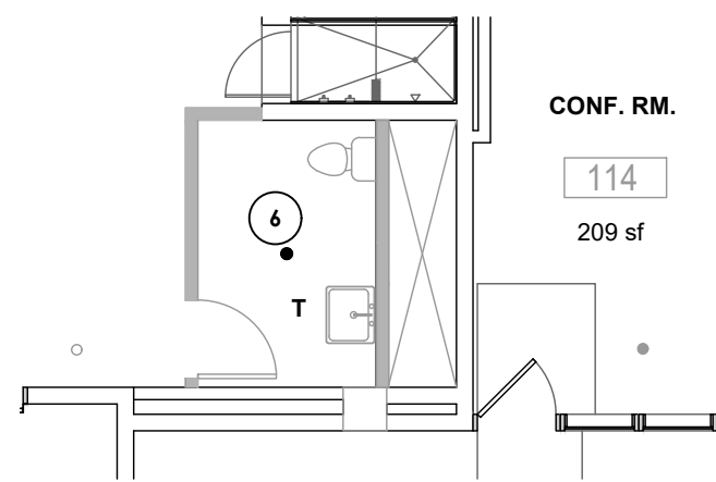
9 NEW 1ST FLOOR TOILET ROOM PLUMBING NEW WORK P201 SCALE: 1/8" = 1'-0"
