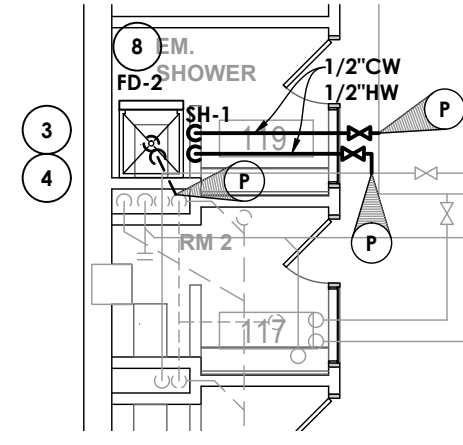
1 EMERGENCY SHOWER PLUMBING NEW WORK P201 SCALE: 1/8" = 1'-0"
