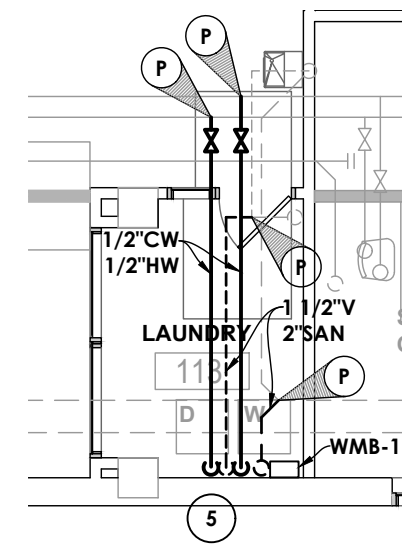
2 LAUNDRY 113 PLUMBING NEW WORK P201 SCALE: 1/8" = 1'-0"
