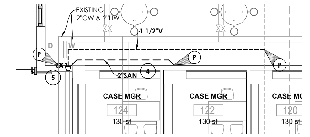
4 LAUNDRY PLUMBING NEW WORK P201 SCALE: 1/8" = 1'-0"
