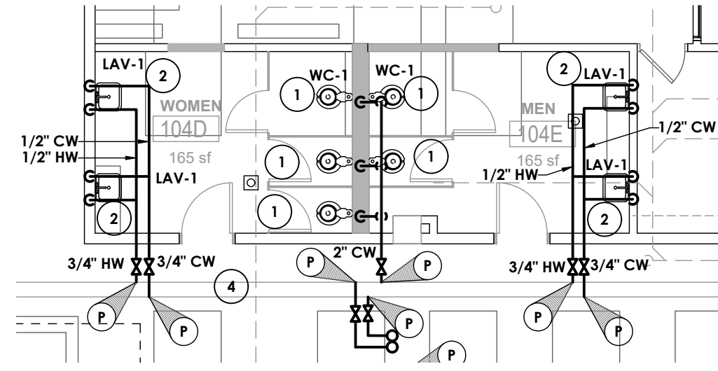
6 104D & 104E DOMESTIC WATER NEW WORK P201 SCALE: 1/8" = 1'-0"
