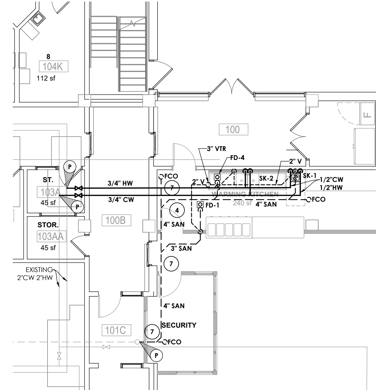
7 WARMING KITCHEN PLUMBING NEW WORK P201 SCALE: 1/8" = 1'-0"
