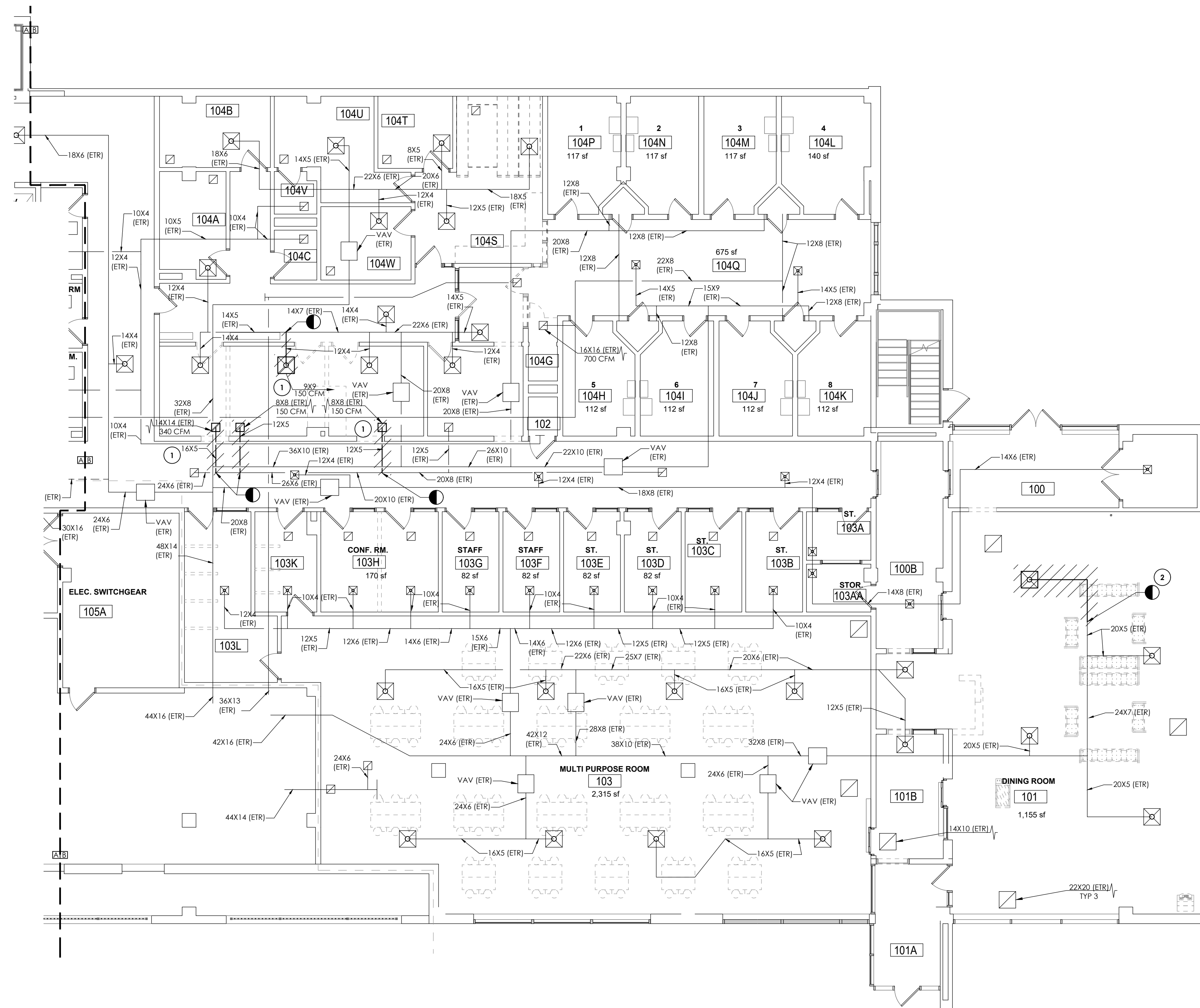
1 FIRST FLOOR MECHANICAL DEMOLITION PLAN, SOUTH H101B SCALE: 1/8" = 1'-0"
