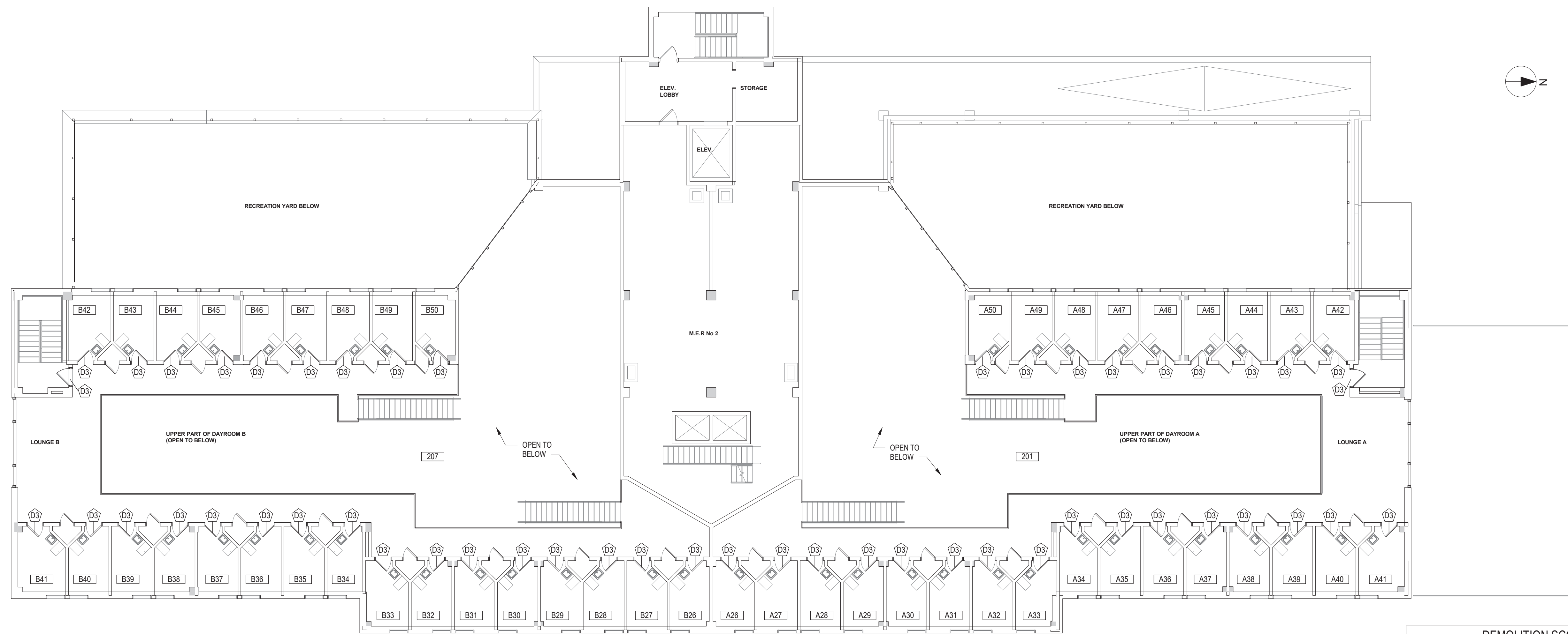
1 THIRD FLOOR PLAN - SELECTIVE DEMOLITION 3/32" = 1'-0" 0 5 15 35 FT
